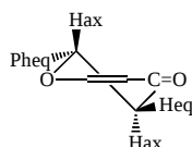
Figure 1. Quasi chair conformation of the flavanone ring.
