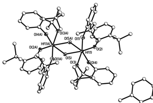
Figure 5. Structure plot of \text{OC}_6\text{H}_4(\text{C}(\text{CH}_3)_3)_2 -2 phenoxide derivative 6 . Thermal ellipsoids of heavy atoms drawn at the 30% level with C atoms drawn as ball and stick for clarity.
