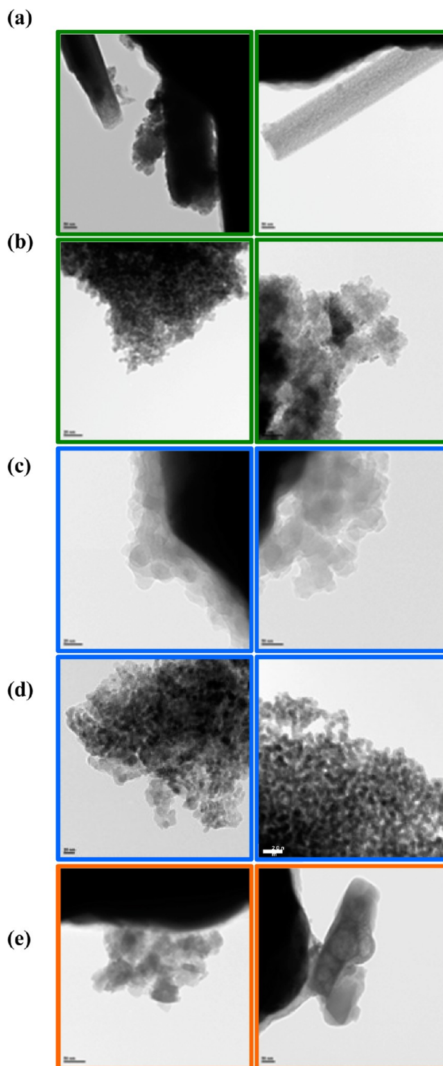
Figure 12. TEM images of nanomaterials generated from (a) \text{Hf}(\text{OBU}^t)_4 (scale bar = 50, 50 nm), (b) 8 [ \text{OC}_6\text{H}_3(\text{CH}_3)_2\text{-2,6} ; 20, 50 nm], (c) 19a [ \text{OC}_6\text{H}_3(\text{CH}(\text{CH}_3)_2\text{-2,6} ; 20, 50 nm], (d) 22 (OTHF; 20, 20 nm), and (e) 25 (THME; 50, 50 nm) after annealing at 650 °C in air.
