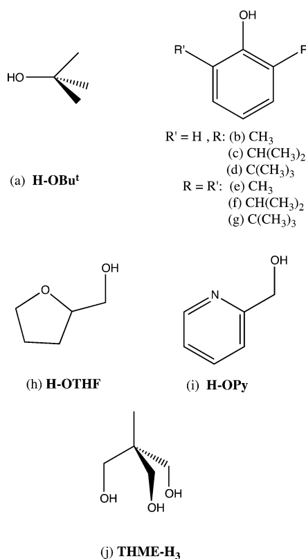
Figure 1. Schematic representation of the various ligands employed in this study: (a) HOC(CH_3)_3 ( HOBu^t ), HOC_6H_3(R)-2, (R')-6 where R' = H and R = (b) CH_3 , (c) CH(CH_3)_2 , and (d) C(CH_3)_3 , HOC_6H_4(R)-2, (R')-6 where R' = R = (e) CH_3 , (f) CH(CH_3)_2 , (g) C(CH_3)_3 , (h) (OC_4H_7)^{cy}(CH_2OH)-2 ( H-OTHF ), (i) (NC_5H_4)^{cy}(CH_2OH)-2 ( H-OPy ), and (j) (HOCH_2)_3CCH_3 ( THME-H_3 ).
