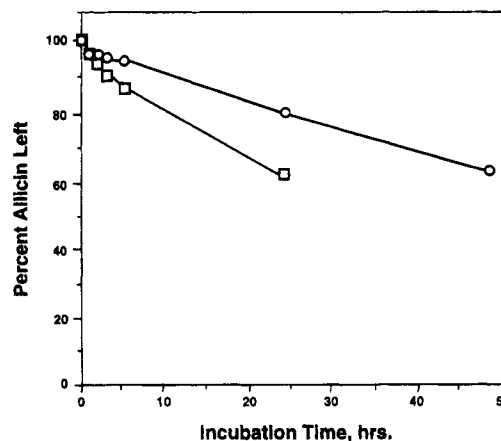
Figure 3. Allicin (1) stability in water at gastric (1.2) and intestinal (7.5) pH at 37^{\circ}\text{C} ; (○) pH 1.2; (□) pH 7.5. Percent allicin (1) remaining was calculated from the ratios of peak areas of internal standard (IS) and 1. See Figure 2 and Experimental Procedures for HPLC conditions.
