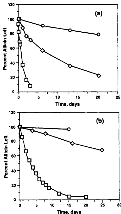
Figure 1. Allicin (1) stability in organic solvents: (○) at -16^{\circ}\text{C} ; (◇) at 6^{\circ}\text{C} ; (□) at room temperature in ethyl acetate (a) and in methanol (b). Percent allicin (1) remaining was calculated by comparison of the ratios of peak areas of internal standard (IS) and 1. See Figure 2 and Experimental Procedures for HPLC conditions.
