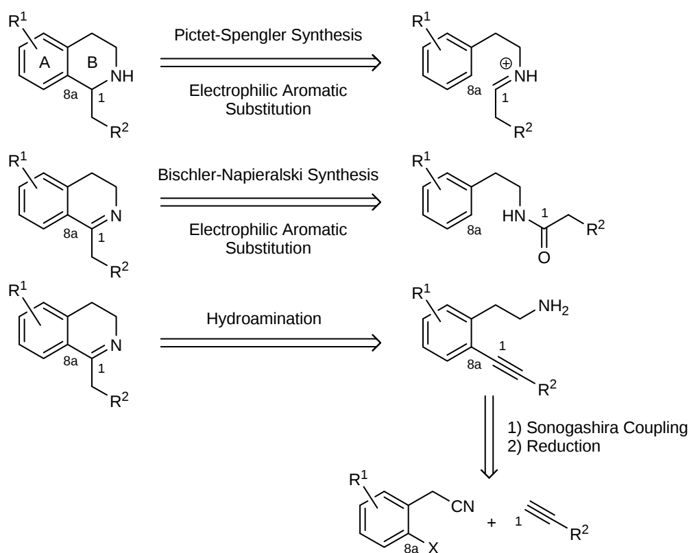
Scheme 1. Retrosynthesis of the benzyloisoquinoline skeleton
