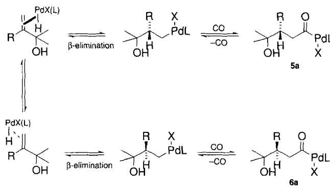
Scheme 3. Proposed mechanism for the hydrocarbonylation of allylic alcohol via a hydridopalladium intermediate (L = (–)-BPPM).
