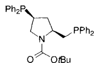
Figure 1. (–)-BPPM.
