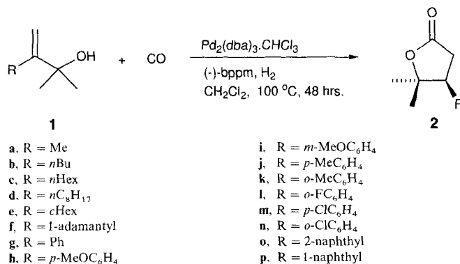
Scheme 1. Palladium-catalyzed asymmetric cyclocarbonylation of allylic alcohols.
