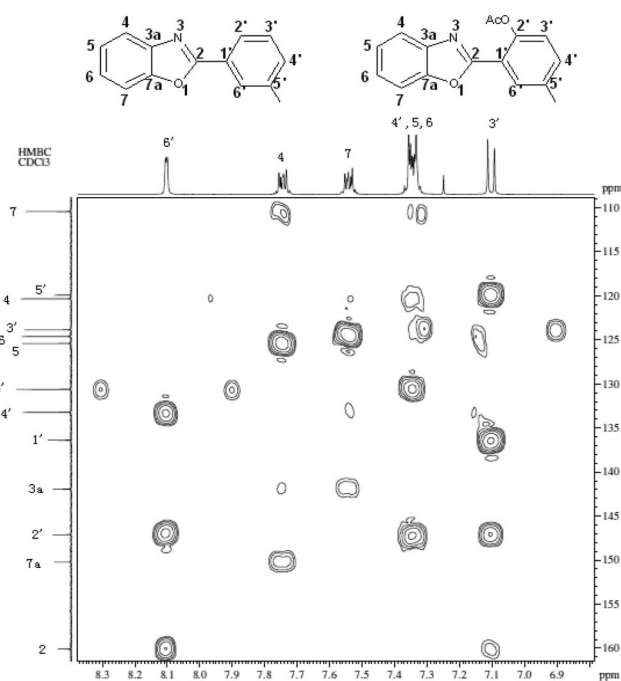
Fig. 3 HMBC spectrum of 3a.
