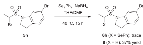
Scheme 4 Attempted selenide displacement resulted in proto-debrominated product.
