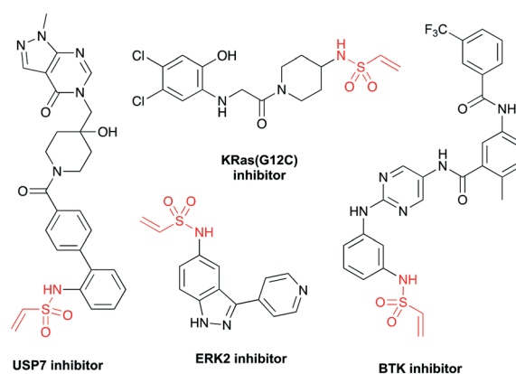
Fig. 1 Structures of terminal vinyl sulfonamide containing protein inhibitors.
