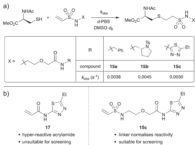
Scheme 7 (a) NMR rate study. Vinyl sulfonamides (10 mM) were reacted with N -acetyl cysteine methyl ester (78 mM) and the rate of reaction monitored by 1 H NMR spectroscopy. (b) Comparison of unlinked and linker thiadiazole fragments for irreversible tethering.
