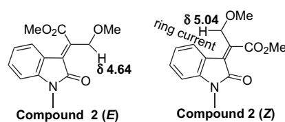
Figure 2. Distinction of E and Z isomers of 2 .
