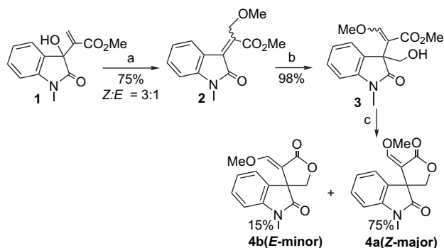
Scheme 2. Synthesis of 3-spiro- \alpha -methylene- \gamma -butyrolactone- N -methyl oxindoles 4a and 4b . (a) \text{CH}(\text{OMe})_3/\text{Mont. K10} , neat, 110 °C, 30 min; (b) aq \text{HCHO} , DABCO, rt, acetone, 1.5 h; (c) PTSA/benzene, 30 min.
