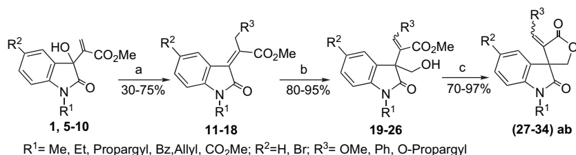
Scheme 3. Synthesis of 3-spiro- \alpha -methylene- \gamma -butyrolactone- N -alkyl oxindoles ( 27a/b – 34a/b ). (a) \text{CH(OMe)}_3 (or) \text{Ar-H} (or) propargyl alcohol/Mont. K10, neat, 110 °C, 30 min; (b) aq HCHO, DABCO, acetone, rt, 2 h; (c) PTSA/benzene, 80 °C, 30 min.
