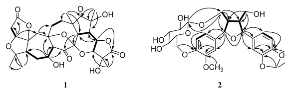
Fig. 2. Selected HMBC ( \rightarrow ) and ^1\text{H} - ^1\text{H} COSY ( \longrightarrow ) Correlations of 1 and 2
