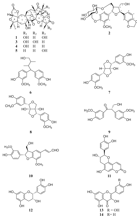
Fig. 1. Structures of Compounds 1–14
