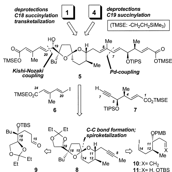
Figure 2. Retrosynthetic analysis of reveromycin A ( 1 ) and B ( 4 ).
