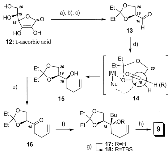
Scheme 1. Synthesis of C15–C20 fragment 9 . a) 0.1 equiv Pd/C (10%), H 2 , H 2 O, 24 h, 55 °C, 96%; b) 1.3 equiv Et 3 C(OEt) 2 , 0.1 equiv CSA, DMF, 48 h, 25 °C, 82%; c) 1.2 equiv KIO 4 , 2.0 equiv KHCO 3 , THF/H 2 O 1:1, 2 h, 23 °C, 85%; d) 1.5 equiv H 2 C=CHCH 2 CH 2 MgBr (2.0 M in THF), THF, –78 to 25 °C, 1 h, 92% (5:1 ratio at C18); e) 2.0 equiv PCC·celite, CH 2 Cl 2 , 25 °C, 2 h, 93%; f) 1.5 equiv BuMgBr (2.0 M in THF), THF, –78 °C, 1.5 h, 95% (4:1 ratio at C18); g) 1.3 equiv TBSOTf, 1.5 equiv 2,6-lutidine, CH 2 Cl 2 , 25 °C, 24 h, 99%; h) O 3 , CH 2 Cl 2 , 20 min, –78 °C; 2.0 equiv Ph 3 P, 95%.
