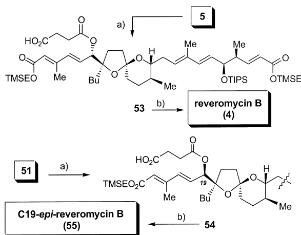
Scheme 10. Completion of the synthesis of reveromycin B ( 4 ) and C19- epi -reveromycin B ( 55 ). a) 10 equiv succinic anhydride, 12 equiv DMAP, 25 °C, 3 h, 85 % for 53 , 88 % for 54 ; b) 10 equiv TBAF · THF, THF, 2 h, 25 °C, 69 % for 4 , 61 % for 55 .
