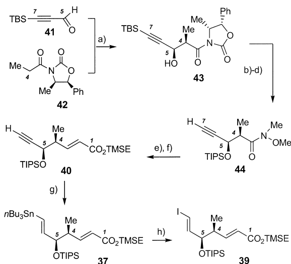
Scheme 6. Synthesis of C1–C7 fragments 37 and 39 . a) 1.0 equiv 42 , 1.0 equiv \text{Bu}_2\text{BOTf} , 1.2 equiv \text{Et}_3\text{N} , then 1.2 equiv 41 , \text{CH}_2\text{Cl}_2 , -78 to 0^\circ\text{C} , 5 h, 80%; b) 9.0 equiv \text{AlMe}_3 , 9.0 equiv \text{MeO-NHMe}\cdot\text{HCl} , THF, -30 to 0^\circ\text{C} , 2 h; c) 2.0 equiv \text{TBAF}\cdot\text{SiO}_2 , THF, 25^\circ\text{C} , 3 h; d) 1.5 equiv \text{TIPSOTf} , 3.0 equiv 2,6-lutidine, \text{CH}_2\text{Cl}_2 , 25^\circ\text{C} , 15 min, 81% (over three steps); e) 2.5 equiv \text{DIBAL-H} (1.5 M in toluene), THF -78^\circ\text{C} , 0.5 h; f) 2.5 equiv \text{Ph}_3\text{P=CH-CO}_2\text{TMSE} ( 45 ), \text{CH}_2\text{Cl}_2 , 25^\circ\text{C} , 15 h, 91% (over two steps); g) 0.02 equiv [\text{Pd}(\text{PPh}_3)_2\text{Cl}_2] , 1.5 equiv n\text{Bu}_3\text{SnH} , benzene, 5^\circ\text{C} , 10 min, 91%; h) \text{I}_2 , \text{CH}_2\text{Cl}_2 , 0^\circ\text{C} , 5 min, 90%.
