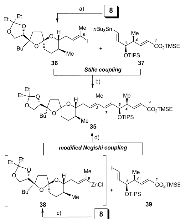
Scheme 7. Synthesis of C1–C20 fragment 35 . a) 1.0 equiv 8 , 2.0 equiv \text{Cp}_2\text{ZrHCl} , benzene, 25^\circ\text{C} , 8 h; \text{I}_2\cdot\text{CCl}_4 (excess), 0^\circ\text{C} , 15 min, 53%; b) 1.0 equiv 36 , 1.0 equiv 37 , 0.05 equiv [\text{Pd}(\text{CH}_3\text{CN})_2\text{Cl}_2] , DMF/THF 1:1, 25^\circ\text{C} , 15 h, 52%; c) 1.0 equiv 8 , 2.0 equiv \text{Cp}_2\text{ZrHCl} , THF, 50^\circ\text{C} , 2 h; 3.0 equiv \text{ZnCl}_2 , THF, 5 min, 25^\circ\text{C} ; d) 1.0 equiv 38 , 1.1 equiv 39 , 0.05 equiv [\text{Pd}(\text{PPh}_3)_4] , THF, 2 h, 25^\circ\text{C} , 84% over two steps.
