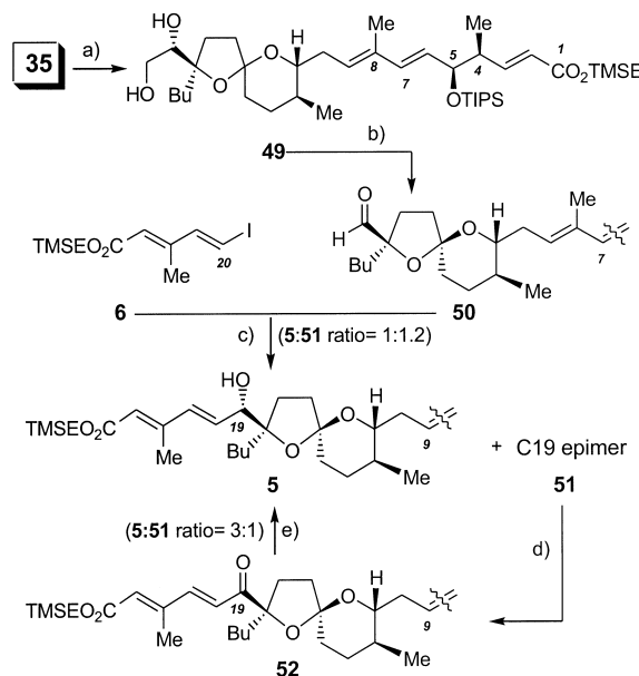
Scheme 9. Synthesis of C1–C24 fragment 5 . a) 3.0 equiv PPTS, MeOH, 3 h, 40 °C, 95 %; b) 6.0 equiv \text{NaIO}_4 , THF/ \text{H}_2\text{O} 2:1, 2 h, 0 °C, 95 %; c) 4.0 equiv 6 , 24 equiv \text{CrCl}_2 (with 0.5 % \text{NiCl}_2 ), DMF, 25 °C, 3 h, 65 % (1.2:1 ratio at C19); d) 1.5 equiv Dess–Martin periodinane, \text{CH}_2\text{Cl}_2 , 2 h, 25 °C, 93 %; e) 5.0 equiv \text{CeCl}_3 \cdot 7\text{H}_2\text{O} , 5.0 equiv \text{LiBH}_4 (2M in THF), THF/MeOH 1:1, –78 to 25 °C, 3 h, 81 %.
