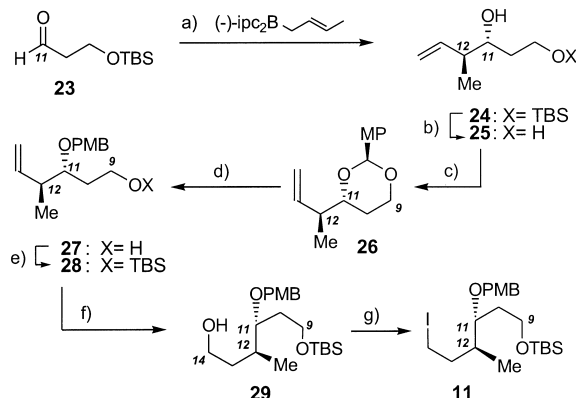
Scheme 3. Synthesis of iodide 11 . a) 1.5 equiv t BuOK, 1.6 equiv trans -2-butene, 1.5 equiv n BuLi, THF, -45^{\circ}\text{C} , 10 min, then 1.6 equiv (-)-\text{ipcb}_2\text{BOMe} (1 M in THF), 2.0 equiv \text{BF}_3 \cdot \text{Et}_2\text{O} , -78^{\circ}\text{C} , 1.0 equiv 23 , 3 h, then 3 N NaOH, 30 % \text{H}_2\text{O}_2 , 25^{\circ}\text{C} , 18 h, 80 %; b) 1.2 equiv TBAF \cdot THF, THF, 25^{\circ}\text{C} , 30 min, 98 %; c) 1.2 equiv \text{PMBCH}(\text{OMe})_2 , 0.1 equiv CSA, \text{CH}_2\text{Cl}_2 , 25^{\circ}\text{C} , 6 h, 98 %; d) 1.5 equiv DIBAL-H (1 M in \text{CH}_2\text{Cl}_2 ), \text{CH}_2\text{Cl}_2 , -78 to 25^{\circ}\text{C} , 2 h, 91 %; e) 2.5 equiv imidazole, 1.3 equiv TBSCl, \text{CH}_2\text{Cl}_2 , 25^{\circ}\text{C} , 1 h, 97 %; f) 1.0 equiv \text{BH}_3 \cdot \text{THF} , -40^{\circ}\text{C} , 10 h, then 3 N NaOH, 30 % \text{H}_2\text{O}_2 , 25^{\circ}\text{C} , 30 min, 85 %; g) 2.4 equiv imidazole, 1.2 equiv \text{Ph}_3\text{P} , 1.2 equiv \text{I}_2 , THF, 0^{\circ}\text{C} , 30 min, 96 %.
