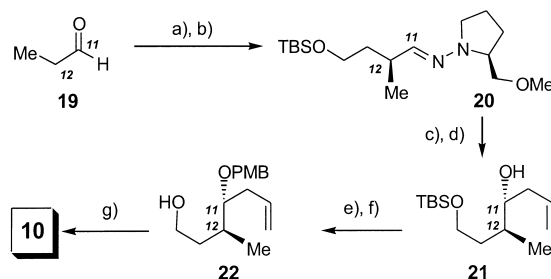
Scheme 2. Synthesis of iodide 10 . a) 1.0 equiv SAMP (neat), 3.0 equiv 19 , 80 °C, 2 h, 92%; b) 1.1 equiv i Pr 2 NH, 1.1 equiv n BuLi (1.6 N in hexanes), THF, 0 °C, 6 h; 1.1 equiv n BuLi (1.6 N in hexanes), –20 °C, 2 h; 2.0 equiv TBSO(CH 2 ) 2 I, –100 to –20 °C, 70%; c) O 3 , CH 2 Cl 2 , –78 °C, 1 h; d) 1.5 equiv (+)-(ipc) 2 B-CH 2 CH=CH 2 (3 M in Et 2 O), Et 2 O, –78 °C, 2 h; 8.0 equiv H 2 O 2 (30%), 13 equiv NaOH (3 N), –78 to 25 °C, 15 h, 78% (over two steps); e) 1.2 equiv KH, 1.5 equiv PMBCl, Et 2 O, 0 °C, 6 h; f) 1.3 equiv TBAF·THF (1 M), THF, 25 °C, 1 h, 81% (over two steps); g) 2.4 equiv imidazole, 1.2 equiv Ph 3 P, 1.2 equiv I 2 , 0 °C, 1 h, 97%.
