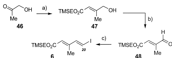
Scheme 8. Synthesis of iodide 6 . a) 1.0 equiv 46 , 1.2 equiv 45 , \text{CH}_2\text{Cl}_2 , 25 °C, 24 h, 85 %; b) 2.1 equiv PCC-celite, \text{CH}_2\text{Cl}_2 , 25 °C, 2 h, 88 %; c) 8.0 equiv \text{CrCl}_2 , 2.5 equiv \text{CHI}_3 , THF, 0 to 25 °C, 0.5 h, 65 %.
