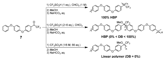
Scheme 2. Synthesis of Hyperbranched Polymers with Controlled Degree of Branching from 0 to 100%
