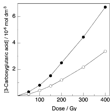
Figure 3. Formation of 3-carboxyglutaric acid as a secondary product in the radiolysis of \text{N}_2\text{O} -saturated acetic acid ( 3 \times 10^{-3} \text{ mol dm}^{-3} ) solutions (●, pH 3.4; ○, pH 7.0). For comparison: at a dose of 50 Gy, the concentration of the primary product succinic acid has reached values of \approx 10^{-5} \text{ mol dm}^{-3} (cf. Figure 2).
