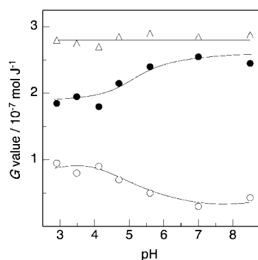
Figure 2. \gamma -Radiolysis of acetic acid in \text{N}_2\text{O} -saturated solution. Yields ( G values) of succinic acid (●), glycolic acid (○), sum (△) of both products.
