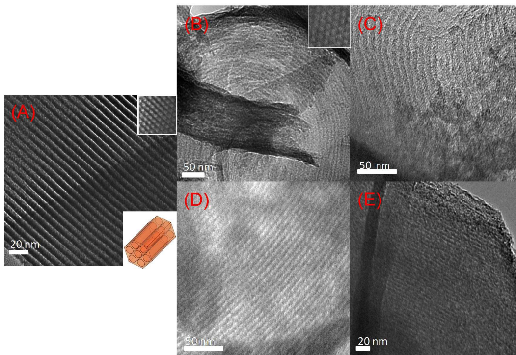
Figure 1. TEM images of SBA-15 (A), NOMC (B), BOMC (C), POMC (D) and OMC (E). The inset of image (A & B, same scale as for the main image) shows a top view of the hexagonal array of rods. All OMC samples were measured after removing the SBA-15 template.
