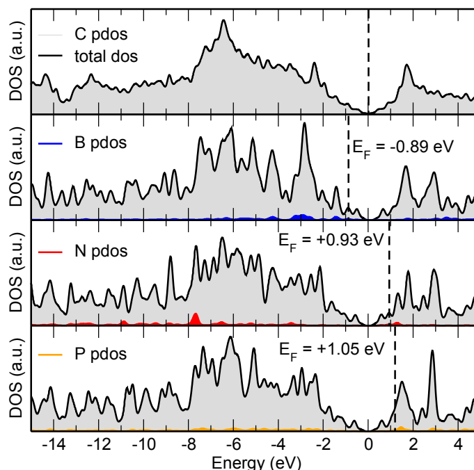
Figure 6. Density of states (DOS) and the projected density of states (PDOS) of pure graphene (top panel) and B-, N- or P-doped graphene with the doping element in graphitic configuration (second, third and fourth panel, respectively).
