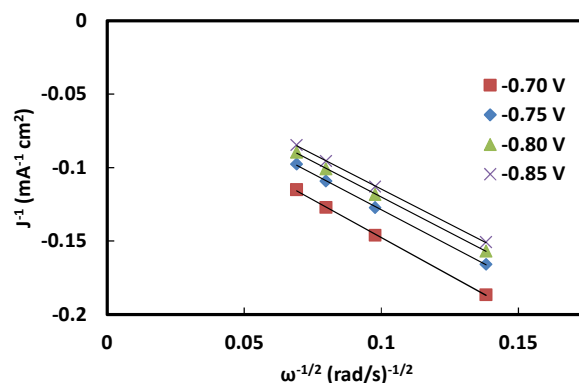
Figure 3. Koutěcký-Levich plots ( J^{-1} vs. \omega^{-1/2} ) of NOMC at a potential interval from -0.70 to -0.85 V vs. \text{Fc}/\text{Fc}^{+} .
