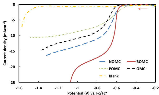
Figure 2. LSV plots of NOMC, BOMC, POMC, OMC and blank NOMC recorded in 5 mM nitrobenzene and 0.3 M \text{HClO}_4 in ethanol at a scan rate of 5 \text{ mVs}^{-1} and with a rotation speed of 2000 rpm and corrected for the iR drop.
