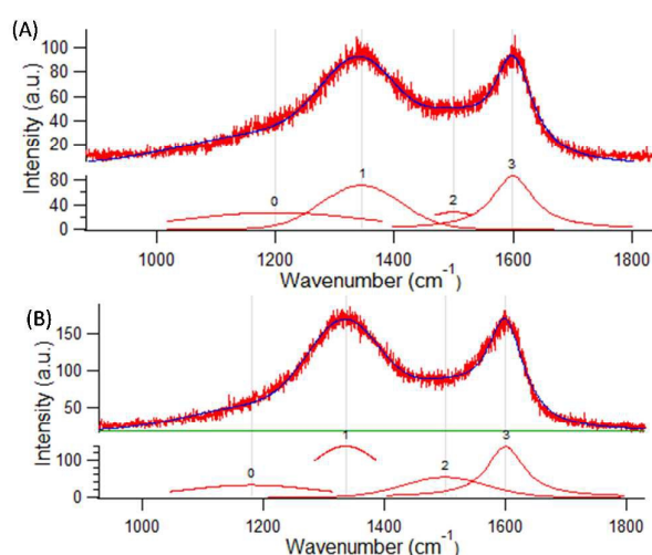
Figure 4. Deconvoluted Raman spectra of BOMC (A) and POMC (B). The Raman spectra of NOMC and OMC can be found in Fig. S6 in the ESI.
