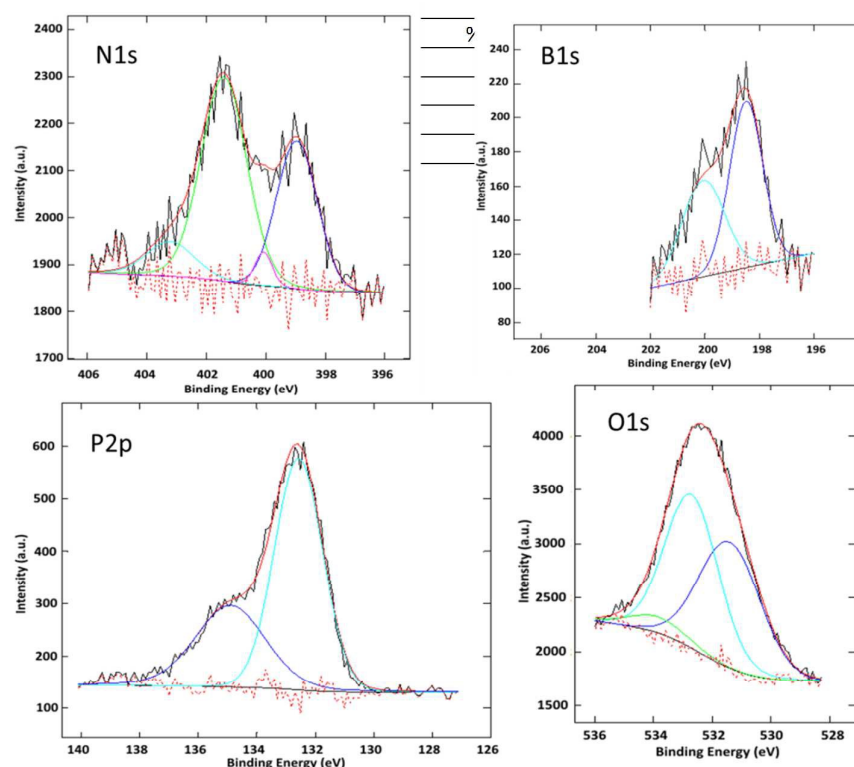
Figure 5. Deconvoluted high resolution N 1s (NOMC), B 1s (BOMC), P 2p (POMC) and O 1s (OMC) XPS signals.
