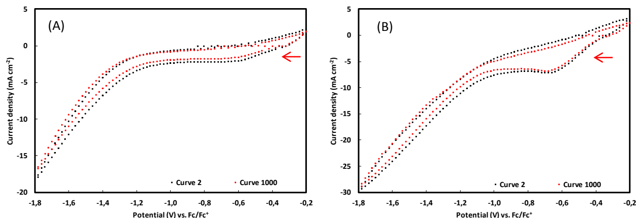
Figure 7. Stability test of (A) NOMC and (B) BOMC by cyclic voltammetry. The potential was cycled between -0.2 and -1.8 V vs. \text{Fc}/\text{Fc}^+ at a scan rate of 100 \text{ mVs}^{-1} . Only the second (after initial stabilisation) and the last curve are presented here. After 999 cycles, the measurement was paused and the solution was stirred to ensure a homogeneous nitrobenzene concentration throughout the medium. Afterwards, the last scan was measured.
