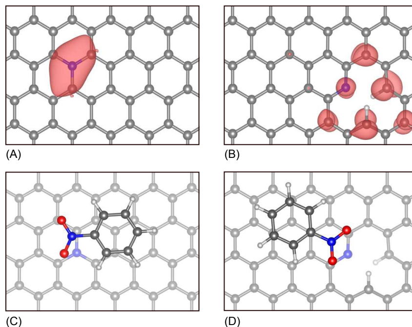
Figure 8. Electronic density isosurfaces of the highest occupied state of N-doped graphene (used to simulate the NOMC surface) in which the N atoms are in graphitic (A) or pyridinic (B) configuration. Ball-and-stick representation of the most stable adsorption geometries of nitrobenzene on N-doped graphene in which the N atoms are in graphitic (C) or pyridinic (D) configuration [grey spheres represent C atoms, red spheres O atoms, blue spheres N atoms and white spheres H atoms].
