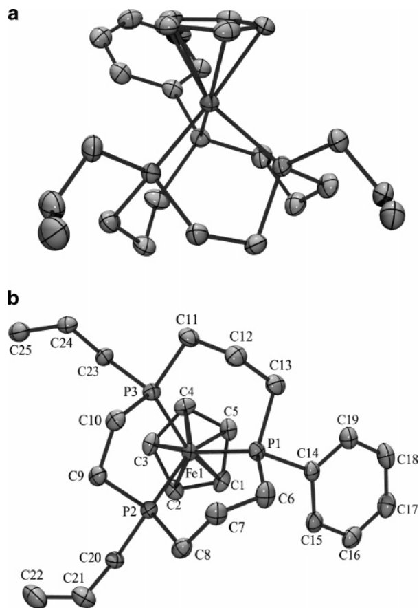
Figure 3. Two views of the crystal structure of the cation of 14 , [(\eta^5\text{-C}_5\text{H}_5)\text{Fe}\{\text{11-aneP}_3\text{-Ph, (C}_3\text{H}_5)_2\}]^+ : (a) approximately parallel to the Cp plane; (b) approximately perpendicular to the Cp plane with the atom-labeling scheme. Ellipsoids are drawn at the 50% probability level. Selected bond lengths (Å): Fe1–C5 2.092(3), Fe1–C3 2.094(4), Fe1–C4 2.100(3), Fe1–C1 2.109(3), Fe1–C2 2.110(3), Fe1–Cp (centroid) 1.722(4), Fe1–P1 2.1943(9), Fe1–P3 2.1954(10), Fe1–P2 2.2026(9), P1–C13 1.835(4), P1–C14 1.849(3), P1–C6 1.857(4), P2–C8 1.834(3), P2–C9 1.844(3), P2–C20 1.844(4), P3–C11 1.833(4), P3–C10 1.840(3), P3–C23 1.848(3), C20–C21 1.498(5), C21–C22 1.309(5), C23–C24 1.499(5), C24–C25 1.309(5). Selected bond angles (deg): P1–Fe1–Cp (centroid) 121.8, P2–Fe1–Cp (centroid) 126.8, P3–Fe1–Cp (centroid) 123.1, P1–Fe1–P3 93.98(4), P1–Fe1–P2 95.93(4), P3–Fe1–P2 85.68(3), C13–P1–Fe1 114.31(12), C14–P1–Fe1 115.71(11), C6–P1–Fe1 121.25(13), C8–P2–Fe1 119.15(12), C9–P2–Fe1 109.28(12), C20–P2–Fe1 119.44(12), C11–P3–Fe1 118.79(12), C10–P3–Fe1 111.50(12), C23–P3–Fe1 115.69(12), C13–P1–C14 101.59(17), C13–P1–C6 102.63(19), C14–P1–C6 98.38(16), C8–P2–C9 102.10(16), C8–P2–C20 102.93(17), C9–P2–C20 101.25(16), C11–P3–C10 104.01(17), C11–P3–C23 102.46(17), C10–P3–C23 102.50(16), C22–C21–C20 125.0(4), C25–C24–C23 124.2(4).
