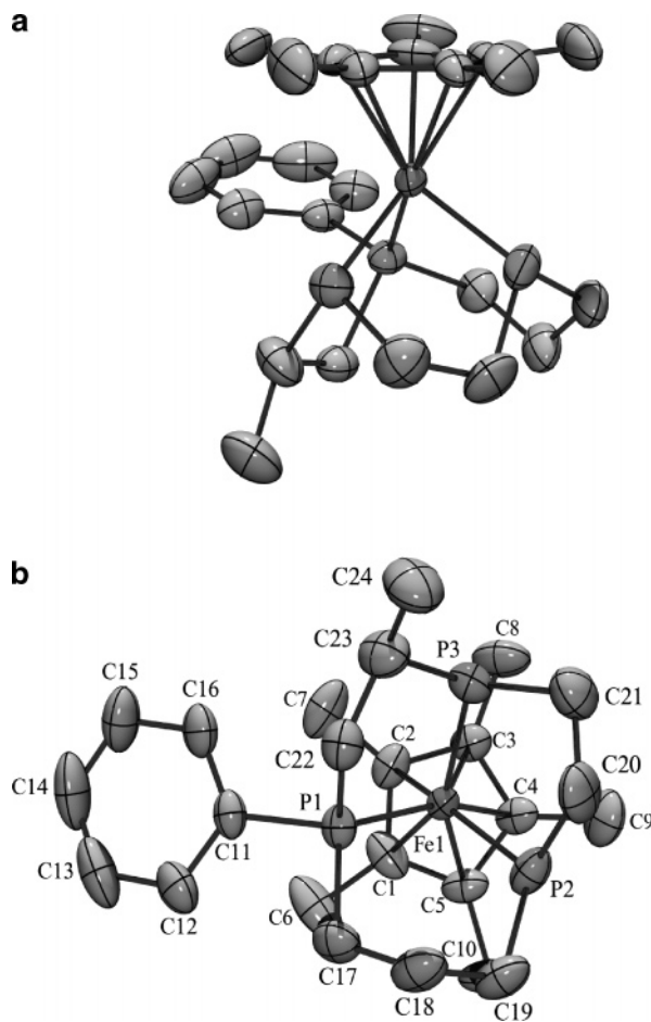
Figure 2. Two views of the crystal structure of the cation of 10a , 1 S ,3 R ,4 R ,8 R ,Fe- [(\eta^5\text{-C}_5\text{Me}_5)\text{Fe}(\text{Me-10-aneP}_3\text{-H}_2, \text{Ph})]^+ : (a) approximately parallel to the Cp* plane; (b) approximately perpendicular to the Cp plane with the atom labeling scheme. Ellipsoids are drawn at the 50% probability level. Selected bond lengths (Å): Fe1–Cp (centroid) 1.728(6), Fe1–P2 2.150(2), Fe1–P3 2.169(2), Fe1–P1 2.195(2), P1–C11 1.833(6), P1–C22 1.841(6), P1–C17 1.853(6), P2–C19 1.821(7), P2–C20 1.853(8), P3–C21 1.812(8), P3–C23 1.864(7), C22–C23 1.505(10), C23–C24 1.514(10). Selected bond angles (deg): P1–Fe1–Cp (centroid) 131.2, P2–Fe1–Cp (centroid) 122.9, P3–Fe1–Cp (centroid) 127.0, P2–Fe1–P3 85.94(8), P2–Fe1–P1 90.06(7), P3–Fe1–P1 85.97(7), C11–P1–C22 101.8(3), C11–P1–C17 102.2(3), C22–P1–C17 102.1(3), C11–P1–Fe1 121.4(2), C22–P1–Fe1 110.6(2), C17–P1–Fe1 116.2(2), C19–P2–C20 104.8(4), C19–P2–Fe1 122.0(3), C20–P2–Fe1 111.6(2), C21–P3–C23 107.9(4), C21–P3–Fe1 110.1(3), C23–P3–Fe1 112.0(2), C22–C23–P3 108.5(5), C24–C23–P3 114.2(6).
