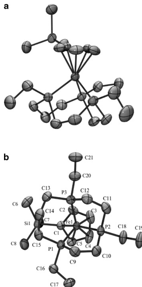
Figure 1. Two views of the crystal structure of the cation of 6 , [(\eta^5\text{-Me}_3\text{SiC}_5\text{H}_4)\text{Fe}(\text{10-aneP}_3\text{-Et}_3)]^+ : (a) approximately parallel to the \text{SiMe}_3\text{Cp} plane; (b) approximately perpendicular to the Cp plane with the atom-labeling scheme. Ellipsoids are drawn at the 50% probability level. Selected bond lengths (Å): Fe1–Cp(centroid) 1.730(6), Fe1–P2 2.1784(10), Fe1–P1 2.1788(10), Fe1–P3 2.1921(10), P1–C16 1.826(4), P1–C15 1.827(4), P1–C9 1.847(4), P2–C18 1.822(4), P2–C10 1.833(4), P2–C11 1.840(4), P3–C20 1.836(4), P3–C13 1.840(4), P3–C12 1.847(4), Si1–C6 1.857(5), Si1–C8 1.860(4), Si1–C7 1.865(4), Si1–C1 1.866(4). Selected bond angles (deg): P1–Fe1–Cp(centroid) 129.0, P2–Fe1–Cp(centroid) 125.0, P3–Fe1–Cp(centroid) 126.8, P2–Fe1–P1 86.50(4), P2–Fe1–P3 85.85(4), P1–Fe1–P3 90.12(4), C16–P1–C15 101.27(19), C16–P1–C9 101.73(19), C15–P1–C9 102.9(2), C16–P1–Fe1 119.36(13), C15–P1–Fe1 117.88(14), C9–P1–Fe1 111.35(13), C18–P2–C10 103.4(2), C18–P2–C11 103.9(2), C10–P2–C11 104.44(19), C18–P2–Fe1 122.29(15), C10–P2–Fe1 111.21(14), C11–P2–Fe1 110.00(15), C20–P3–C13 102.9(2), C20–P3–C12 103.40(19), C13–P3–C12 103.64(19), C20–P3–Fe1 116.55(13), C13–P3–Fe1 118.82(13), C12–P3–Fe1 109.79(14). Torsion angle (deg): C3–C2–C1–Si1 15.7.
