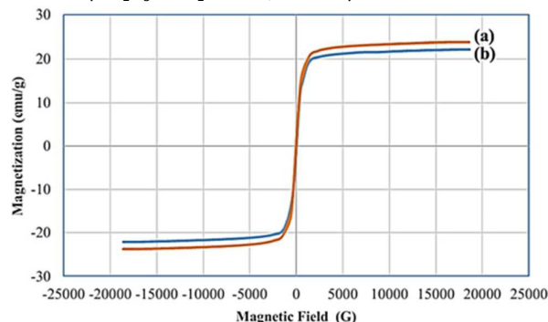
Fig. 6 Magnetization curves of (a) \gamma\text{-Fe}_2\text{O}_3\text{@TiO}_2 nanoparticles (I) and (b) \gamma\text{-Fe}_2\text{O}_3\text{@TiO}_2\text{-EG-Cu}^{\text{II}} .
