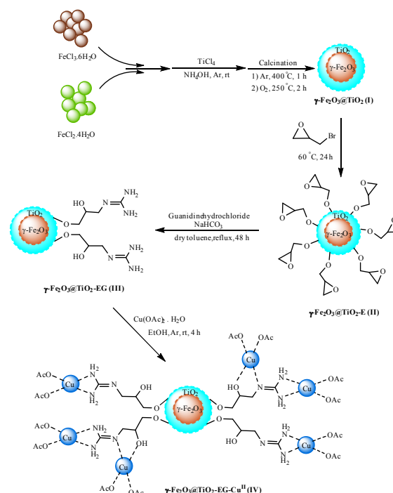
Scheme 1 Preparation of Cu II immobilized on guanidinated epibromohydrin functionalized \gamma -Fe 2 O 3 @TiO 2 ( \gamma -Fe 2 O 3 @TiO 2 -EG-Cu II ).
