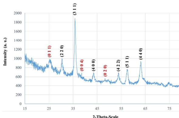
Fig. 4 XRD pattern of \gamma\text{-Fe}_2\text{O}_3\text{@TiO}_2 MNPs.
