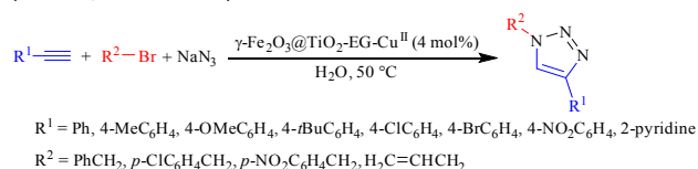
Scheme 2 Synthesis of different structurally 1,4-disubstituted 1,2,3-triazoles in the presence of \gamma\text{-Fe}_2\text{O}_3\text{@TiO}_2\text{-EG-Cu}^{\text{II}} , in water.
