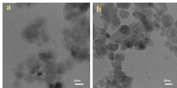
Fig. 3 HRTEM images of \gamma\text{-Fe}_2\text{O}_3\text{@TiO}_2\text{-EG-Cu}^{\text{II}} (a, b).
