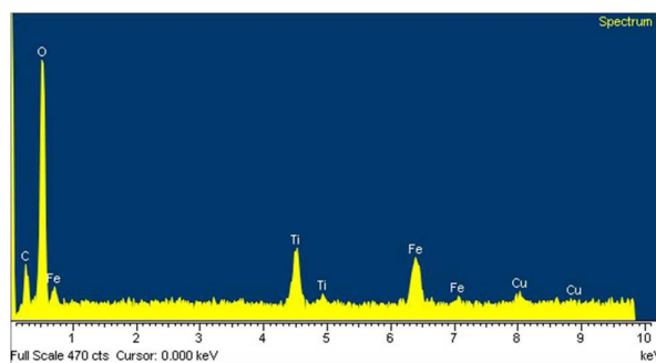
Fig. 5 EDX analysis of \gamma\text{-Fe}_2\text{O}_3\text{@TiO}_2\text{-EG-Cu}^{\text{II}} .
