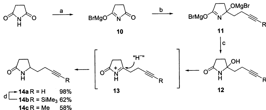
Scheme 1. Reagents and conditions: (a) MeMgBr (1 equiv), THF, 0°C to rt, 1 h; (b) RC + CCH 2 CH 2 MgBr (2 equiv), THF, 0°C to rt, 1 h; (c) NaBH 3 CN, THF/HOAc, pH 3, rt, 1 h; (d) TBAF, THF, 0°C, 30 min.
