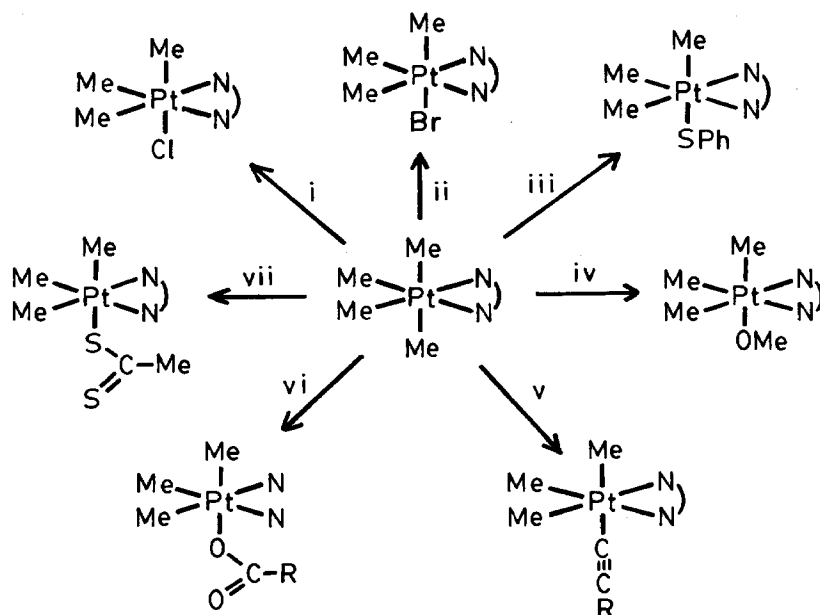
Scheme 1. \text{NN} = 2,2' -bipyridine. Reagents: h\nu (Hg lamp, filtered to give \lambda > 420 \text{ nm} ) and (i) \text{CH}_2\text{Cl}_2 or \text{CHCl}_3 ; (ii) \text{CH}_2\text{BrCH}_2\text{Br} ; (iii) \text{PhSH} ; (iv) \text{MeOH} ; (v) \text{RC}\equiv\text{CH} , \text{R} = \text{Me, Ph} or \text{CH}_2\text{CH}_2\text{OH} ; (vi) \text{RCO}_2\text{Me} , \text{R} = \text{H, Me, CH=CH}_2 or \text{C}\equiv\text{CCO}_2\text{Me} ; (vii) \text{CS}_2 . The solvent was the reagent, acetone or benzene and isolated yields were at least 80%.
