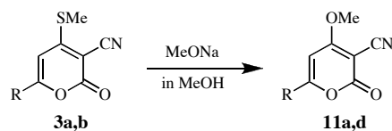
Scheme 3. Synthesis of 6-aryl-4-methoxy-2-oxo-2 H -pyran-3-carbonitriles.
