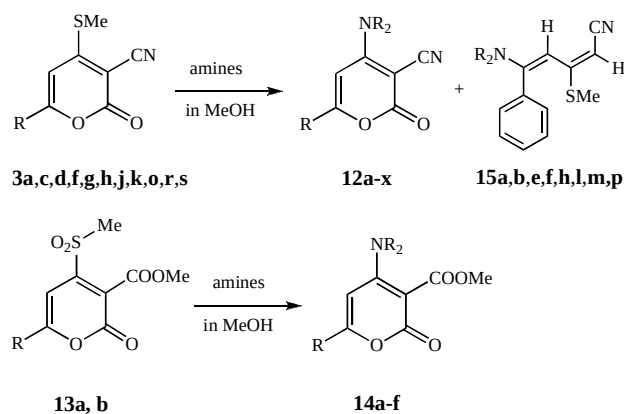
Scheme 4. Synthesis of 4-Amino-6-aryl-2-oxo-2H-pyrans.
