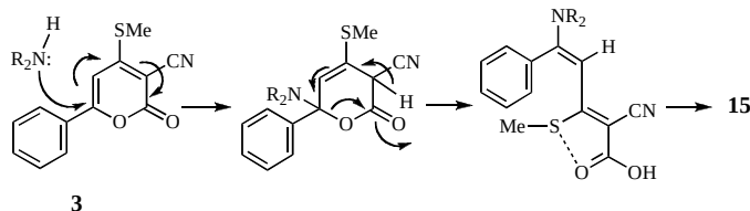
Scheme 5. Reaction Pathway of 15
