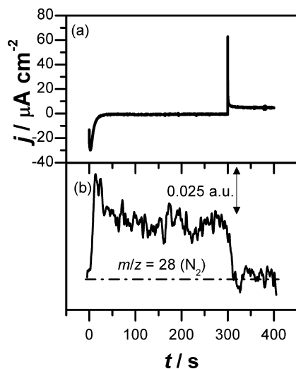
Figure 2. Chronoamperometric profile during OLEMS measurements (A) and ion current profiles for m/z = 28 (B) in 0.1 M NaOH containing 2 mM \text{NaNO}_2 . The working electrode was a Pt(100) electrode, \nu = 1 mV/s. The electrode was kept at 0.55 V for 300 s, followed by a potential step to 0.65 V. The m/z current immediately before t = 0 is also shown.
