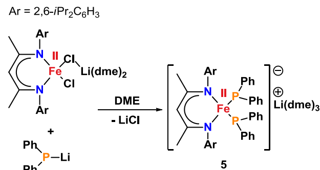
Scheme 3. Synthesis of complex 5 .
