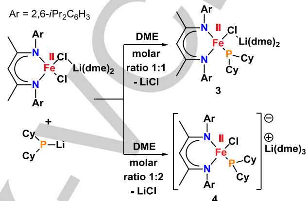
Scheme 2. Syntheses of complexes 3 and 4 .
