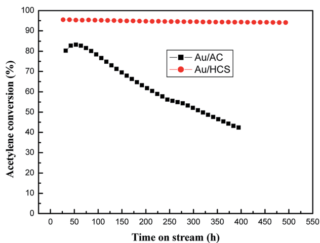
Fig. 7 Long lifetime testing of Au/AC and Au/HCS catalysts (GHSV = 360 \text{ h}^{-1} , V_{\text{HCl}}/V_{\text{C}_2\text{H}_2} = 1.15 , reaction temperature = 180^\circ\text{C} ).
