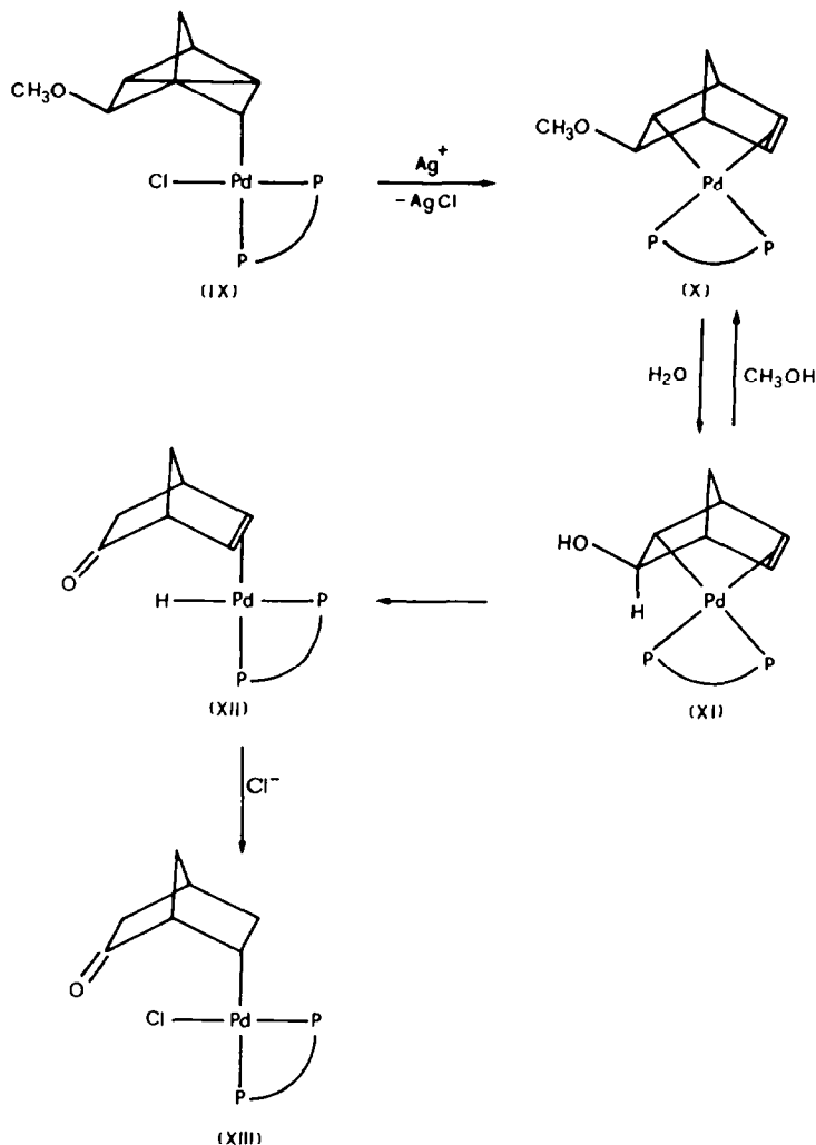
SCHEME 2
