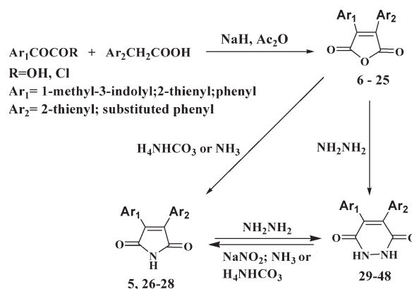
Scheme 1. Synthesis of diaryl-substituted maleic anhydrides, imides, and hydrazides.
