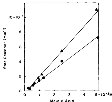
Figure 5 —Hydrolysis of I in dioxane at 37°C; water, 2 M. Plot of the two consecutive rate constants versus maleic acid concentration. Key: ( \Delta ) k_{H^+} ; ( \bullet ) k_f .
