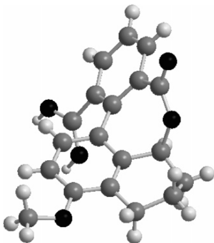
Figure 2. Molecular structure of motor 1 . The Chem 3D structure of ( S )- 1 (in a racemic mixture) using coordinates obtained by X-ray crystallography. The Chem 3D structure is shown to clearly illustrate the lowest-energy conformation with M axial chirality.
