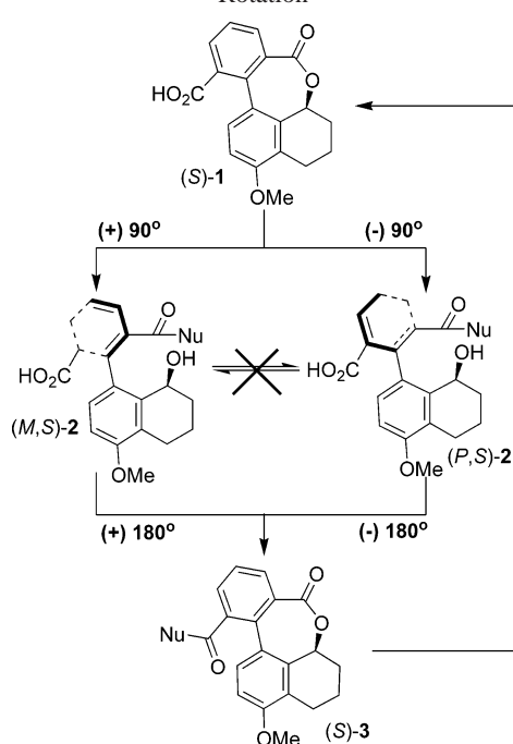
Scheme 1. Proposed Iterative Directed Aryl–Aryl Bond Rotation
