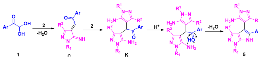
Scheme 4. Proposed Mechanism for the Synthesis of Product 5
