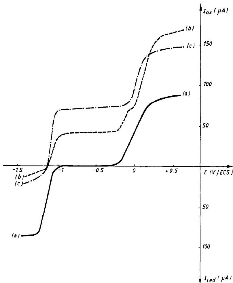
Fig. 2. Linear voltammogram in NMP with \text{NBu}_4\text{BF}_4 ( 10^{-1} M ), at a rotating gold microelectrode ( 3 \text{ mm}^2 ), under argon of: curve a : a mixture of \text{Nibpy}_3(\text{BF}_4)_2 ( 10^{-2} M ) and \text{Nibpy}(\text{CO})_2 ( 10^{-2} M ), this latter having been formed by electroreduction (6 F/Ni) of \text{Nibpy}_3(\text{BF}_4)_2 under \text{CO}_2 ; curve b : same mixture after an electricity intake of 2 F/Ni at -1.2 \text{ V/SCE} ; curve c : after an intake of 2 F/Ni, at -1.2 \text{ V/SCE} in the presence of additional ( 10^{-1} M ) bipyridine.
