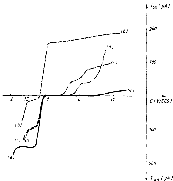
Fig. 3. Linear voltammogram in NMP with \text{NBU}_4\text{BF}_4 ( 10^{-1} \text{ M} ) at a rotating gold microelectrode ( 3 \text{ mm}^2 ) of: curve a : \text{Nibpy}_3(\text{BF}_4)_2 ( 2 \times 10^{-2} \text{ M} ) under argon; curve b : after an electricity intake of 2 F/Ni at -1.2 \text{ V} under argon; curve c : after addition of \text{PhCH}_2\text{Br} ( 2 \times 10^{-2} \text{ M} ) (oxidation of (\text{PhCH}_2)_2\text{Nibpy} ) curve d : after bubbling of CO (oxidation of \text{Nibpy}(\text{CO})_2 , formation of (\text{PhCH}_2)_2\text{CO} ).
