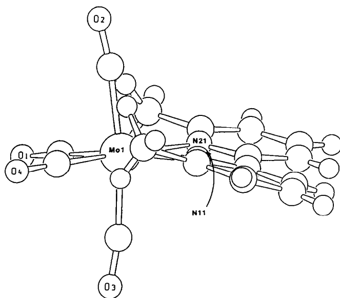
Fig. 2. View of [\text{Mo}(\text{CO})_4(6,6'\text{-Me}_2\text{-2,2'-bipy})] showing the orientation of ligand relative to \{\text{Mo}(\text{CO})_4\} group [12].
