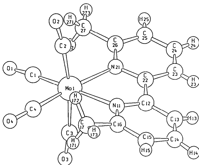
Fig. 1. Molecular structure of [\text{Mo}(\text{CO})_4(6,6'\text{-Me}_2\text{-2,2'-bipy})] with atom numbering scheme [12].
