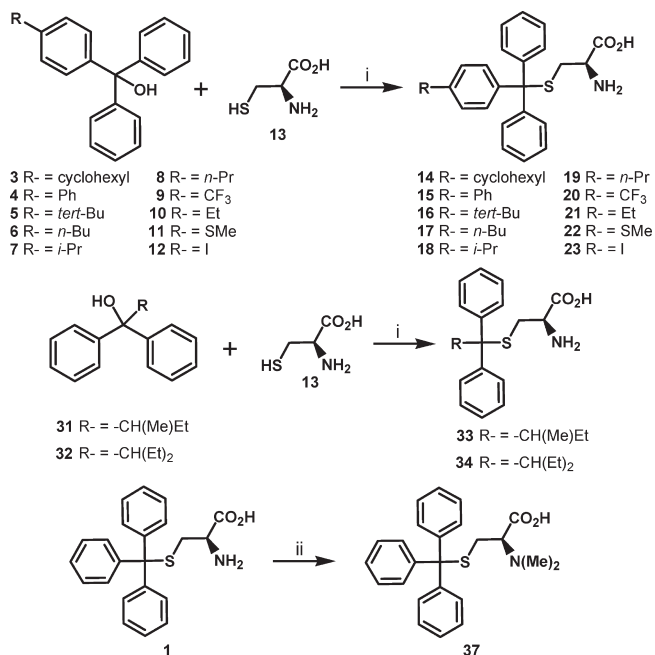
Scheme 1 a
