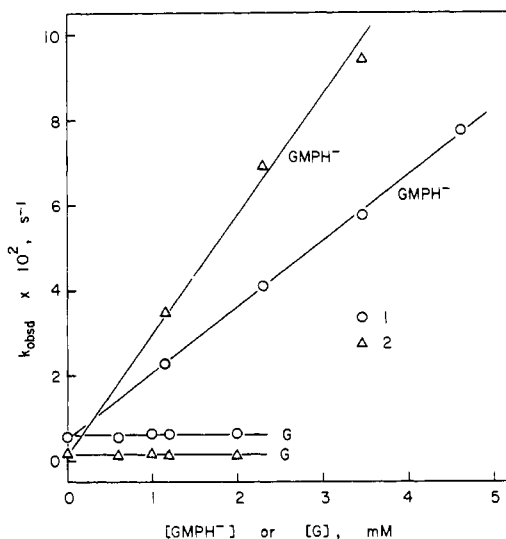
Figure 1. Plots of k_{\text{obsd}} vs. [\text{GMPPH}^-] ( 4 ) or [\text{G}] ( 6 ) for hydrolysis of 1 and 2 in 10% dioxane–water solutions at 25 °C, \mu = 0.1 ( \text{NaClO}_4 ), pH 6.32. 12b The solutions of G also contained 10^{-3} M cacodylic acid buffer for maintenance of pH.
