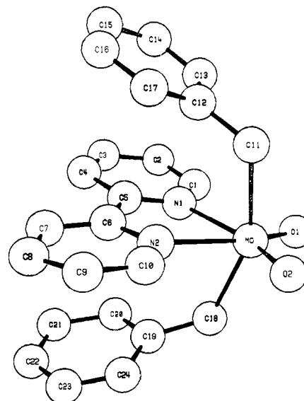
Figure 1. Perspective view of \text{Mo}(\text{O})_2(\text{CH}_2\text{C}_6\text{H}_5)_2(\text{bpy}) with the atoms numbered.
