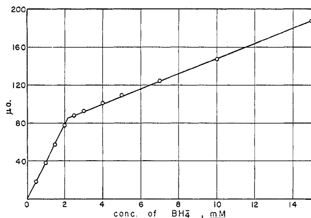
Figure 1.—Dependence of current at -0.01 v. on concentration of \text{NaBH}_4 . Supporting electrolyte: 0.10\text{ }M \text{KCl} , 0.010\text{ }M \text{NaOH} ; capillary characteristics: 1.71\text{ mg.}^{2/3}\text{ sec.}^{-1/2} .
