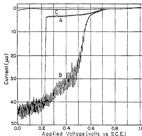
Figure 2.—Illustration of the "scan effect." Test solution: 0.005\text{ }M \text{NaBH}_4 , 0.001\text{ }M \text{NaOH} , 0.10\text{ }M \text{KCl} , 0.01\% gelatin. A: positive-going applied voltage; B: negative-going applied voltage.
