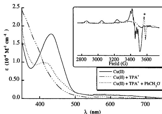
Figure 3. Electronic spectra for Cu II 1 , its oxidized product (1 equiv of TPA + ), and the lithium benzenemethoxide adduct in toluene at -80 °C. Inset: EPR spectra for 1.1 mM Cu II 1 and its oxidized product in toluene/acetonitrile solvents. Instrumental parameters: microwave power, 13 dB; microwave frequency, 9.505 GHz; modulation amplitude, 10 G; temperature, 77 K. The asterisk (*) denotes excess (TPA + ). are used, only Cu II 1 displays catalytic behavior [9.2(± 0.8) turnovers], consistent with the consumption of all oxidizing equivalents (eq 1). 24
