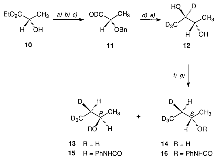
Scheme 3
