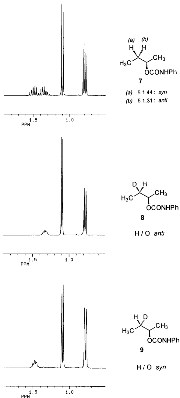
Fig. 2. ^1\text{H} -NMR Spectra (300 MHz, \text{C}_6\text{D}_6 , 303 K) of 1-methylpropyl phenylcarbamate ( 7 ; one enantiomer being represented for clarity) and of its (2- ^2\text{H}_1 )-derivatives 8 and 9
