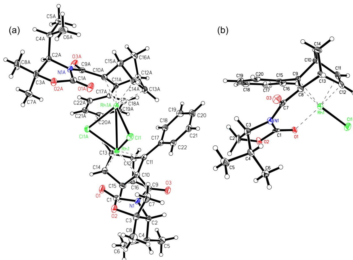
Figure 1. Structure of complexes [\text{RhCl}(\mathbf{6b})]_2 (a) and [\text{RhCl}(\mathbf{5b})] (b) in the solid state. The absolute configuration was determined by anomalous dispersion with relevant Flack parameters x = -0.031(6) and 0.01(3) , respectively. For getting better overall standard deviations of the geometric parameters of the [\text{RhCl}(\mathbf{6b})]_2 X-ray structure, a severely disordered \text{Et}_2\text{O} solvate molecule was removed with SQUEEZE as implemented in PLATON. [48] The \text{Rh1}\cdots\text{O1} and \text{Rh1}-\text{Cl1} distances in [\text{RhCl}(\mathbf{5b})] are shorter than in [\text{RhCl}(\mathbf{6b})]_2 and interactions of \text{C8}=\text{C9} , \text{C11}=\text{C12} to Rh elongate the double bonds.
