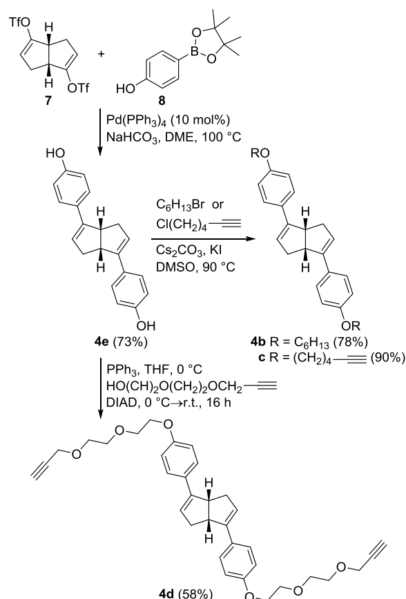
Scheme 2. Synthesis of novel chiral bicyclo[3.3.0.]octadiene ligands 4 . For details see Supporting Information.
