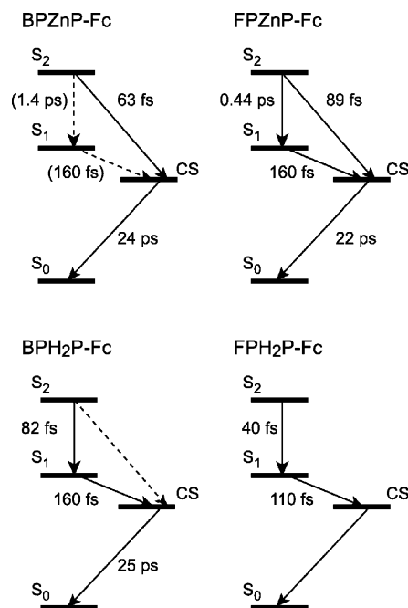
Figure 9. Reaction scheme after Soret excitation of the XP–Fc s . The primary and secondary reaction pathways are shown as solid and dashed arrows, respectively. The data for FPH 2 P–Fc were obtained from ref 20.
