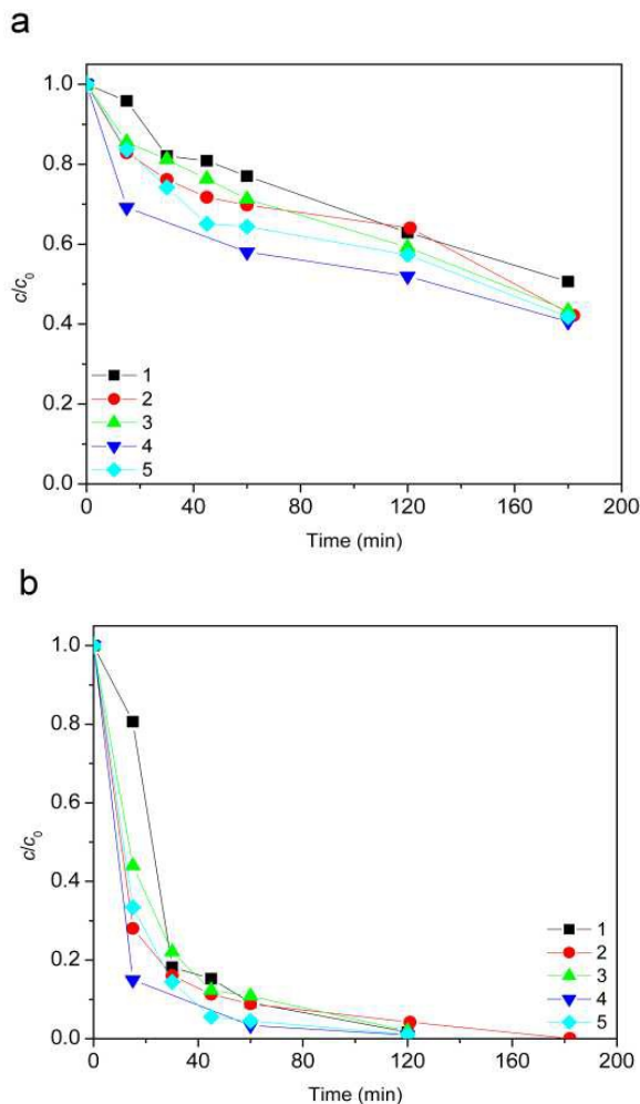
Fig. 8 Evolution of ionic liquid ( c_0 = 0.38 \text{ mmol L}^{-1} ) degradation along the time using SS radiation: a) [bmim] + and b) [Sal] - . Water matrix: (1) tap water; (2) condensate water; (3) pond water; (4) river water; (5) rain water. Other reaction conditions: 7.2Fe/TiO 2 (1.67 g L -1 ) + 45 mmol L -1 H 2 O 2 + 70 μL h -1 H 2 O 2 at pH 2.8.
