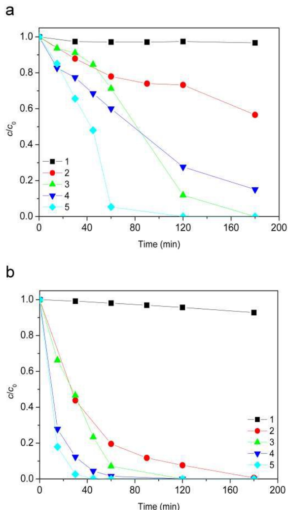
Fig. 4 Evolution of ionic liquid ( c_0 = 0.38 \text{ mmol L}^{-1} ) degradation along the time using UVA radiation: a) [\text{bmim}]^+ and b) [\text{Sal}]^- . Applied AOPs: (1) direct photolysis at pH 2.8; (2) 4.5 \times 10^{-2} \text{ mol L}^{-1} \text{ H}_2\text{O}_2 + 70 \mu\text{L h}^{-1} \text{ H}_2\text{O}_2 at pH 2.8; (3) \text{TiO}_2 \text{ P25} ( 1.67 \text{ g L}^{-1} ); (4) 7.2\text{Fe}/\text{TiO}_2 ( 1.67 \text{ g L}^{-1} ) + 4.5 \times 10^{-2} \text{ mol L}^{-1} \text{ H}_2\text{O}_2 + 70 \mu\text{L h}^{-1} \text{ H}_2\text{O}_2 at pH 2.8; (5) \text{TiO}_2 \text{ P25} ( 1.67 \text{ g L}^{-1} ) + 4.5 \times 10^{-2} \text{ mol L}^{-1} \text{ H}_2\text{O}_2 + 70 \mu\text{L h}^{-1} \text{ H}_2\text{O}_2 .
