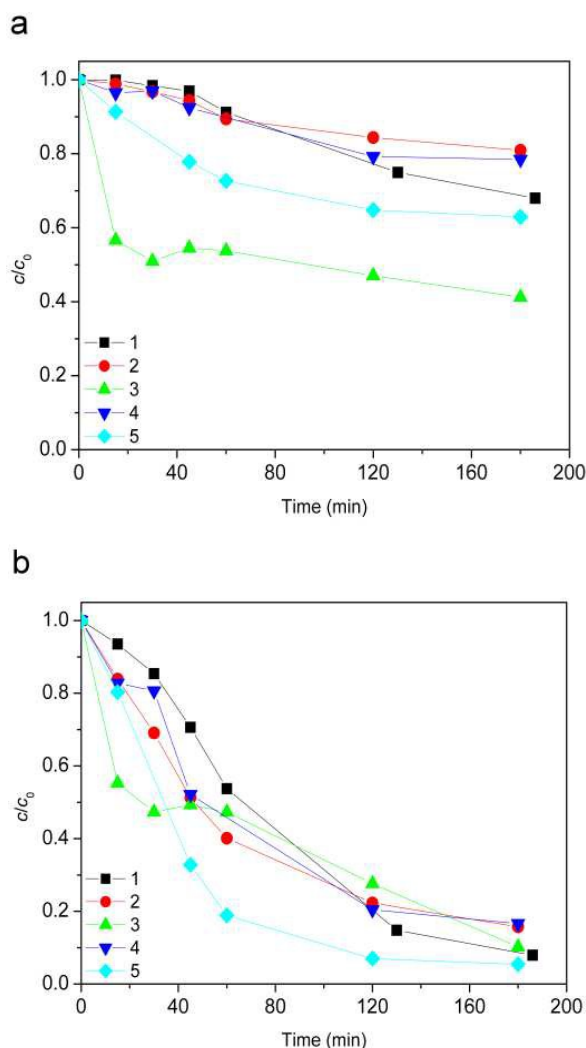
Fig. 7 Evolution of ionic liquid ( c_0 = 0.38 \text{ mmol L}^{-1} ) dark conversion along the time: a) [\text{bmim}]^+ and b) [\text{Sal}]^- . Water matrix: (1) tap water; (2) condensate water; (3) pond water; (4) river water; (5) rain water. Other reaction conditions: 7.2\text{Fe}/\text{TiO}_2 ( 1.67 \text{ g L}^{-1} ) + 45 \text{ mmol L}^{-1} \text{ H}_2\text{O}_2 + 70 \mu\text{L h}^{-1} \text{ H}_2\text{O}_2 at pH 2.8.
