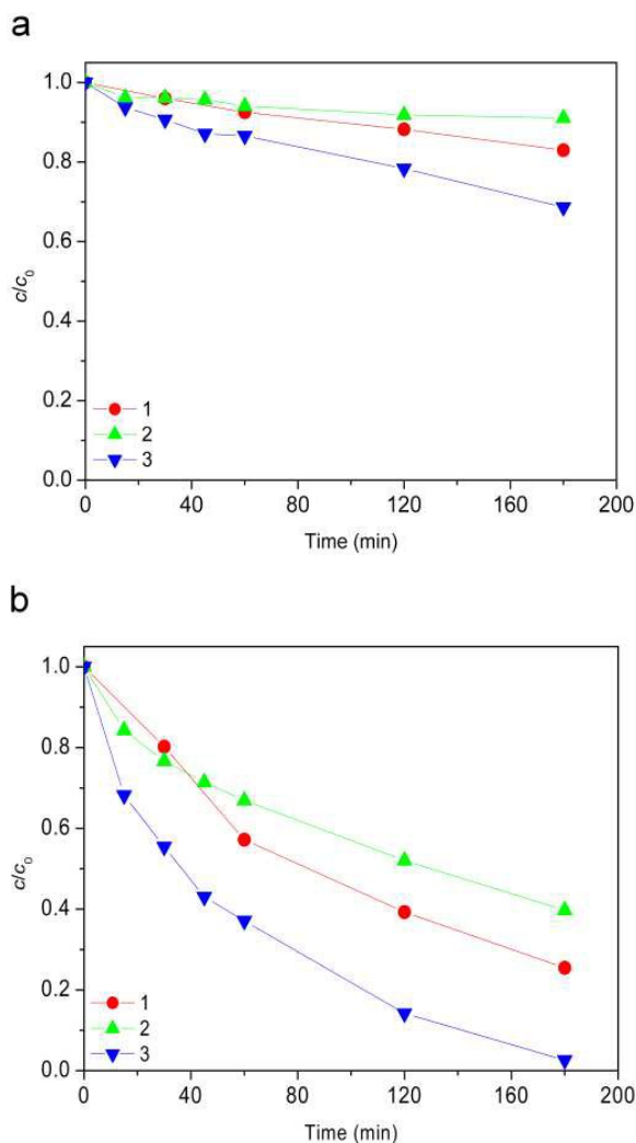
Fig. 5 Evolution of ionic liquid ( c_0 = 0.38 \text{ mmol L}^{-1} ) degradation along the time using SS radiation: a) [\text{bmim}]^+ and b) [\text{Sal}]^- . Applied AOPs: (1) 45 \text{ mmol L}^{-1} \text{ H}_2\text{O}_2 + 70 \mu\text{L h}^{-1} \text{ H}_2\text{O}_2 at pH 2.8; (2) \text{TiO}_2 \text{ P25} ( 1.67 \text{ g L}^{-1} ); (3) 7.2\text{Fe}/\text{TiO}_2 ( 1.67 \text{ g L}^{-1} ) + 45 \text{ mmol L}^{-1} \text{ H}_2\text{O}_2 + 70 \mu\text{L h}^{-1} \text{ H}_2\text{O}_2 at pH 2.8.
