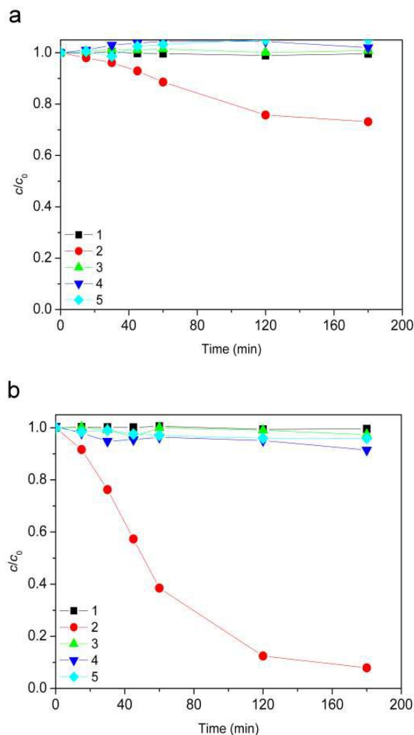
Fig. 3 Evolution of ionic liquid ( c_0 = 0.38 \text{ mmol L}^{-1} ) dark conversion along the time: a) [bmim] + and b) [Sal] - . Reaction conditions: (1) 45 mmol L -1 H 2 O 2 + 70 μL h -1 H 2 O 2 at pH 2.8; (2) 7.2Fe/TiO 2 (1.67 g L -1 ) + 45 mmol L -1 H 2 O 2 + 70 μL h -1 H 2 O 2 at pH 2.8; (3) TiO 2 support (1.67 g L -1 ) + 45 mmol L -1 H 2 O 2 + 70 μL h -1 H 2 O 2 at pH 2.8; (4) TiO 2 P25 (1.67 g L -1 ) + 45 mmol L -1 H 2 O 2 + 70 μL h -1 H 2 O 2 at pH 2.8; (5) 7.2Fe/TiO 2 (1.67 g L -1 ) at pH 2.8.
