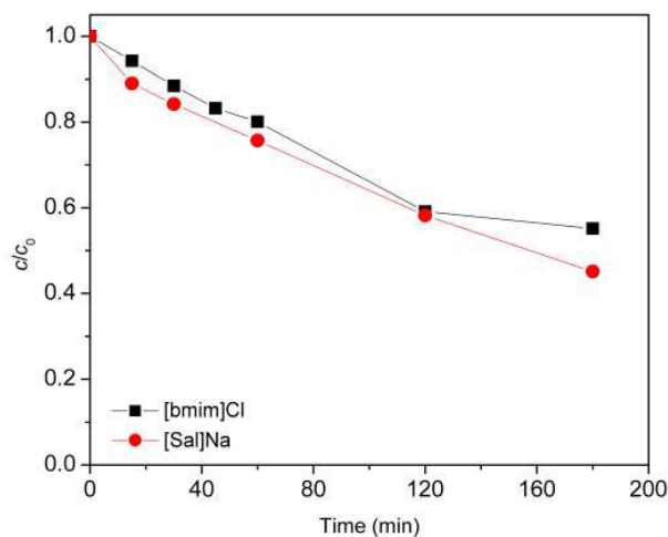
Fig. 6 Photodegradation of [\text{bmim}]\text{Cl} and [\text{Sal}]\text{Na} ( c_0 = 0.38 \text{ mmol L}^{-1} ) using SS radiation and \text{TiO}_2 P25 ( 1.67 \text{ g L}^{-1} ) along the time.
