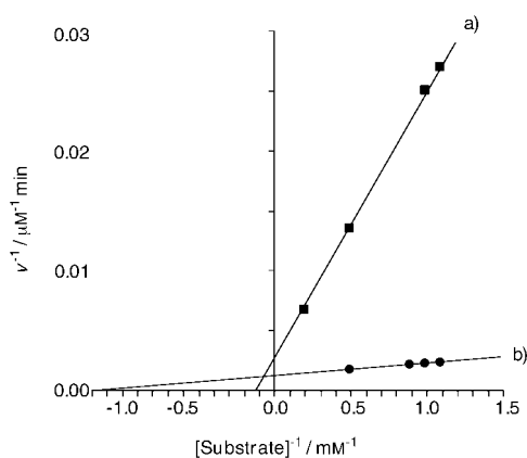
Figure 9. Lineweaver–Burk plots for the oxidation of pyrogallol as a function of substrate (pyrogallol) in the presence of a) the complex of antibody 12E11G with \text{Fe}^{\text{III}} -TMPyP and b) HRP.
