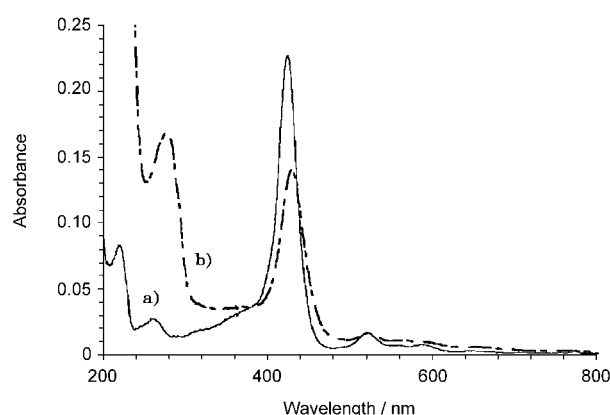
Figure 1. Absorption spectra of TMPyP in a) the absence and b) the presence of anti-3MPy1C antibody (12E11G).
