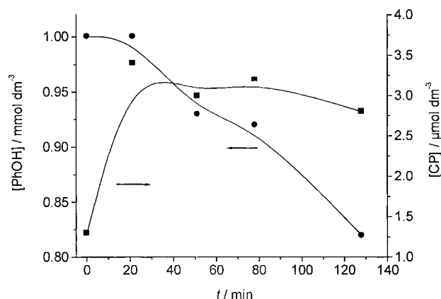
Figure 6. Phenol degradation (●) and 4-CP formation (■) at 1 % PtCl 4 /P25 ( \lambda_{\text{irr}} > 455 nm). [Pt] total = 25 μM, [Cl] total = 100 μM.
