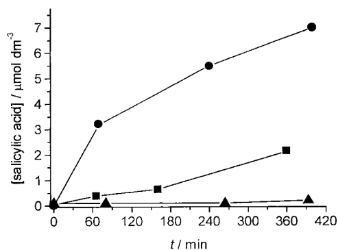
Figure 5. Formation of salicylic acid upon irradiation of 1 % PtCl 4 /P25 in aerated suspension in the presence of benzoic acid ( \lambda_{\text{irr}} > 400 nm, ■); in Ar-saturated suspension in the presence of C(NO 2 ) 4 ( \lambda_{\text{irr}} > 400 nm, ▲) and \lambda_{\text{irr}} > 335 nm, ●). For details see text.
