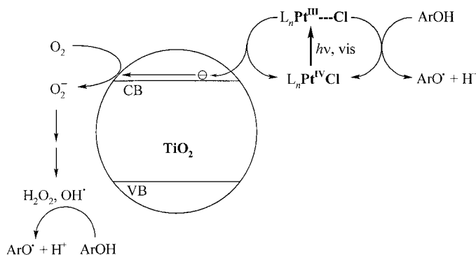
Scheme 1. Proposed mechanism of TiO 2 sensitization by [Pt IV Cl x ] 4−x complexes. CB and VB denote conduction and valence band edge, respectively.
