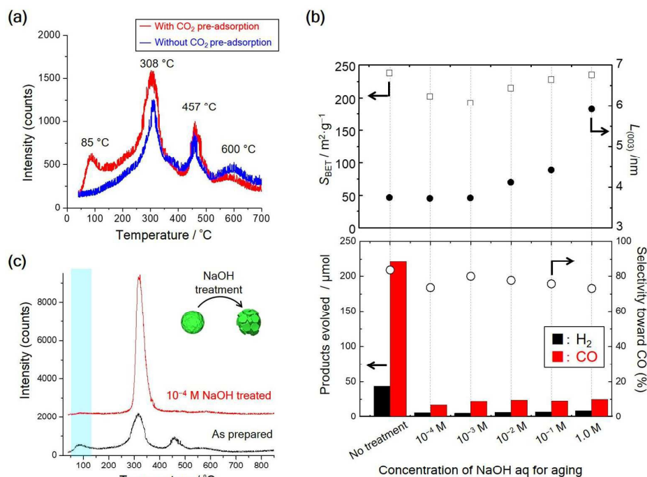
Figure 3. (a) \text{CO}_2 -TPD curves of NLDH-2 with and without preliminary adsorption of \text{CO}_2 . (b) Amounts of gaseous products and reaction selectivity for the reduction of \text{CO}_2 over NLDH-2 after various post treatments. The catalytic reaction was performed for 5 h. BET surface area, S_{\text{BET}} , and 003 crystallite size, L_{(003)} , for NLDH-2 after various aging treatments. (c) \text{CO}_2 -TPD curves of NLDH-2 before and after 10^{-4} M NaOH treatment.
