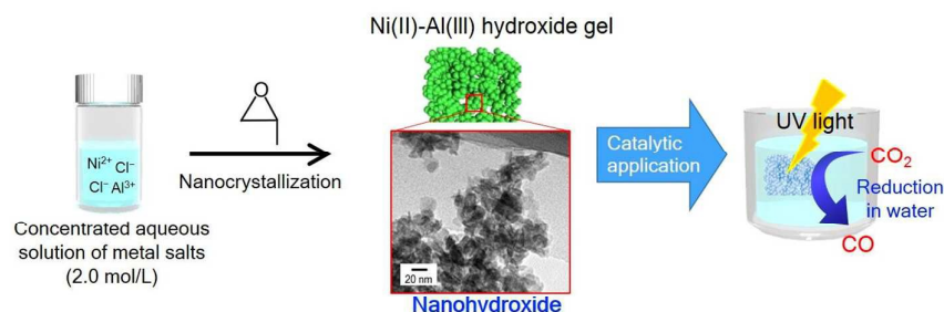
Figure 1. Schematic illustration of the synthesis and photocatalytic application of nano LDH. TEM image showing typical nanostructure of nano LDH prepared at Ni/Al = 2 (NLDH-2 in Table S1).
