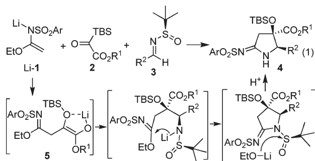
Scheme 1. Silyl Glyoxylates-Mediated Cascade Reaction for the Synthesis of Chiral Cyclic N -Sulfonylamidines
