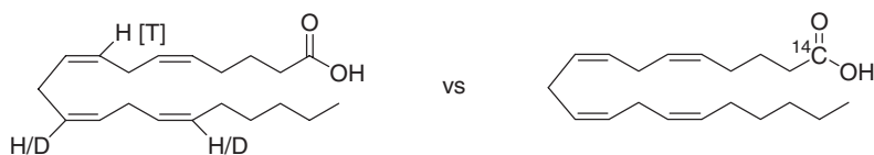
Figure 1. Competitive experiment for measuring secondary kinetic isotope effects
