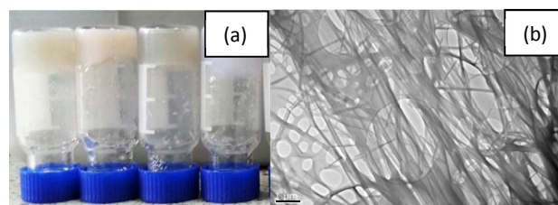
Figure 3 (a) Vial Inversion Screen of linifanib and its fluorinated analogues (left to right: linifanib (1) and linifanib analogues 2, 3 and 4) (b) Transmission Electron Micrograph (TEM): 0.5% (w/v) linifanib in 5% (v/v) DMSO/water; scale bar = 1 \mu m
