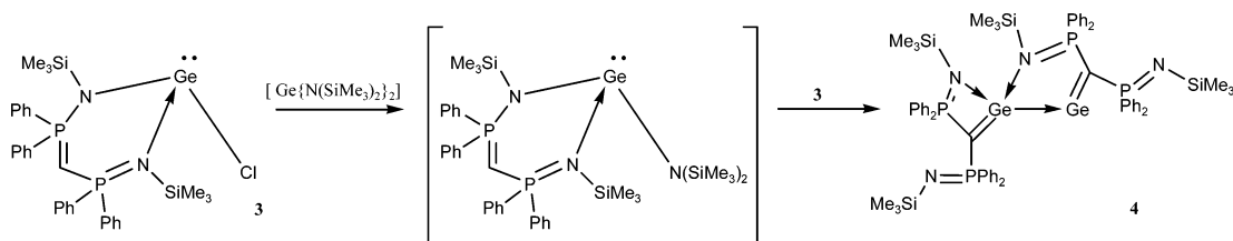
Scheme 3
