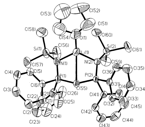
Figure 1. Crystal structure of 2 with atomic numbering scheme.
