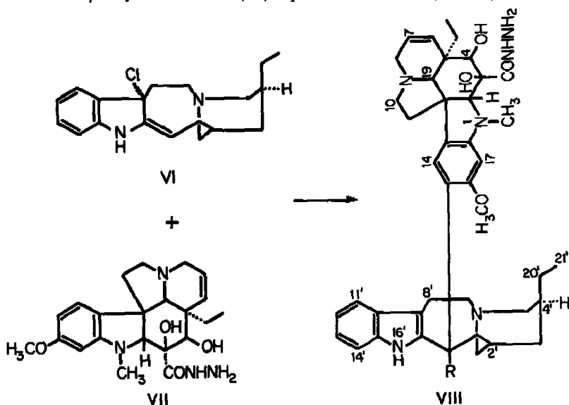
Scheme 2. Coupling of deacetylvindoline hydrazide (VII) with the chloroindolenine derivative of 4 \beta -dihydrocleavamine (VI) to provide dimer VIII (R = H)
