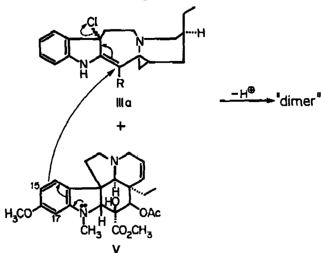
Scheme 1. A proposal outlining the possible coupling of IIIa with vindoline (V) to provide a dimeric product
