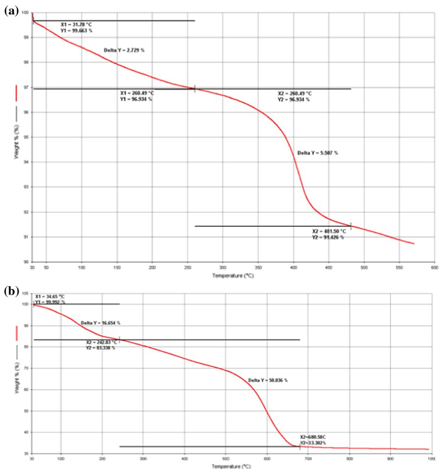
Fig. 3 The TG curves: a \text{Fe}_3\text{O}_4 @nicotinic acid; b \text{Fe}_3\text{O}_4 @nicotinic acid@sulfonic acid chloride nanoparticles
