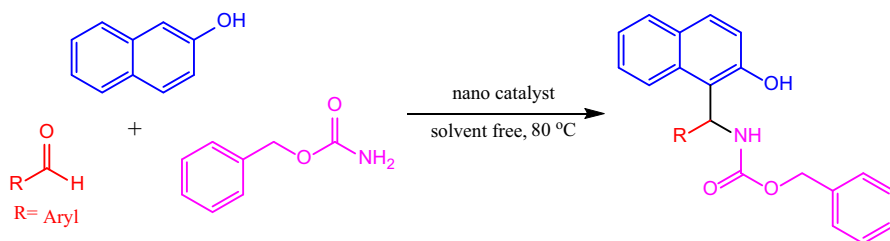
Scheme 1 The preparation of 1-carbamato-alkyl-2-naphthols by nano catalyst
