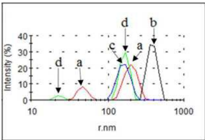
Fig. 4 DLS measurement of the size distributions of the gemini surfactant b at different concentrations: a. 5 times the CMC (red); b. 50 times the CMC (black); c. 100 times the CMC (blue); d. 50 times the CMC (0.1M NaCl) (green).
