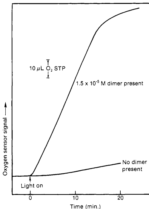
Figure 9. Visible-light-induced oxygen generation in the presence and absence of 1.5 \times 10^{-5} M \text{Ru}^{\text{III}}\text{--O--Ru}^{\text{III}} in 10-mL aqueous 0.1 M phosphate buffer, pH 7, at 25 °C with 1 \times 10^{-4} M \text{Ru}(\text{II})\text{tris}(4,4'\text{-dicarboxy-2,2'-bipyridine}) as a photosensitizer and 5 \times 10^{-3} M \text{S}_2\text{O}_8^{2-} as a sacrificial electron acceptor.
