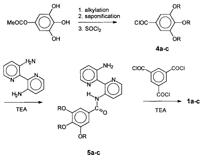
Scheme 1. Synthesis of disc-shaped compounds 1a–c ( R = n\text{-C}_6\text{H}_{13} ( a ), n\text{-C}_{12}\text{H}_{25} ( b ), n\text{-C}_{18}\text{H}_{37} ( c )).
