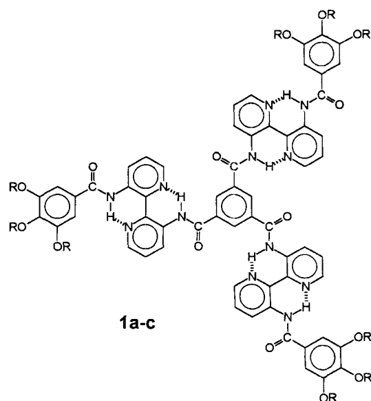
Figure 1. Disc-shaped compounds based on N -acylated 2,2'-bipyridine-3,3'-diamine ( R = n\text{-C}_6\text{H}_{13} ( a ), n\text{-C}_{12}\text{H}_{25} ( b ), n\text{-C}_{18}\text{H}_{37} ( c )).
