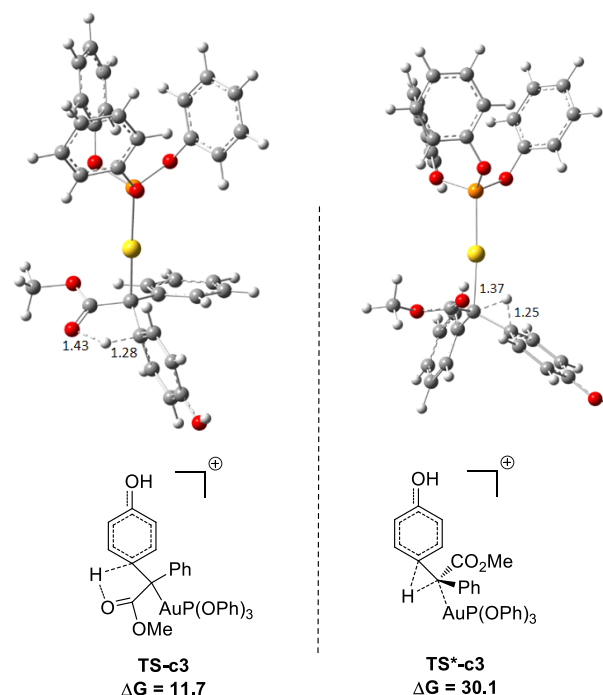
Figure 2. Optimized structures of transition states TS-c3 and TS*-c3 corresponding to Figure 1. The distances are in the units of angstroms and the values of free energies \Delta G are in kcal/mol.
