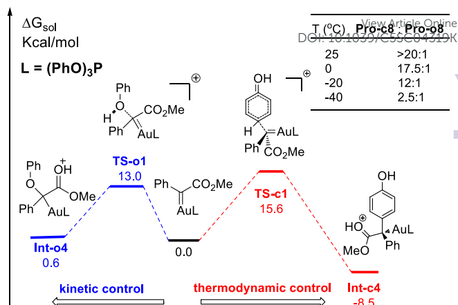
Figure 6. The reaction temperature on the chemoselectivity and the competitive pathways for the formation of two key intermediates. All values of free energies are relative to the reactants of gold carbene and phenol and in the units of kcal/mol.
