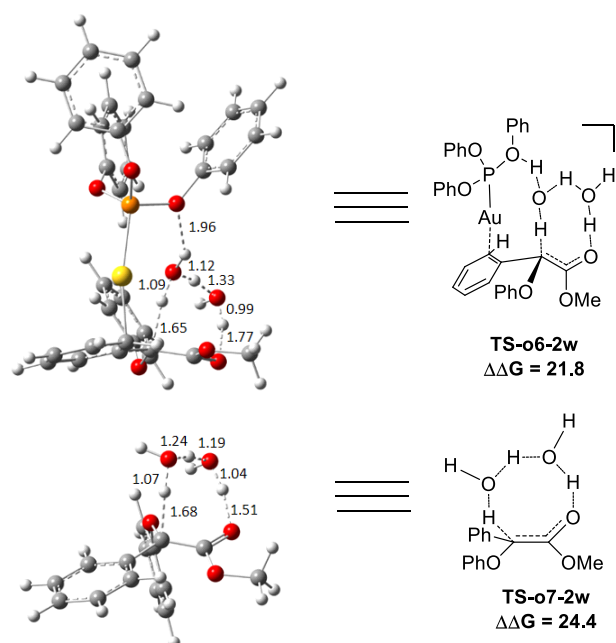
Figure 5. The structures of TS-o6-2w and TS-o7-2w in the proposed O-H functionalization of phenols catalysed by (\text{PhO})_3\text{PAuSbF}_6 . The distances are in the units of angstroms and the values of free energy barriers \Delta\Delta G are in kcal/mol.
